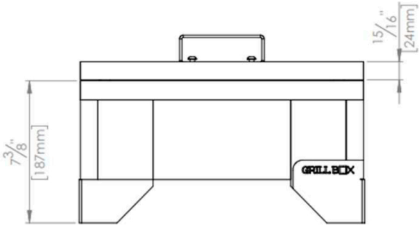
VISTA FRONTAL
